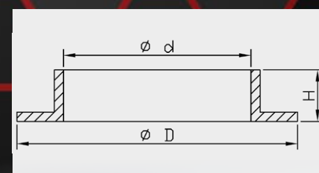
Spring Seat Against Free Piston dimensions
