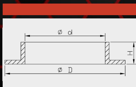
Washer dimensions
