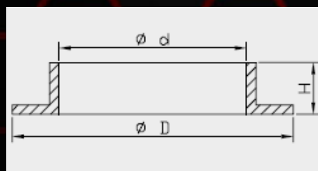
Washer Seal Head Large / Oil Lock dimensions
